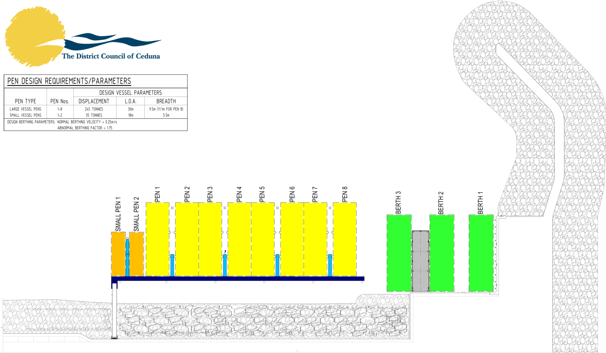
Thevenard Marina Facility - Marina Pen and Wharf Berth Plan
